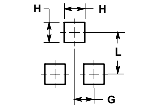
RECOMMENDED PATTERN OF SOLDER PADS
